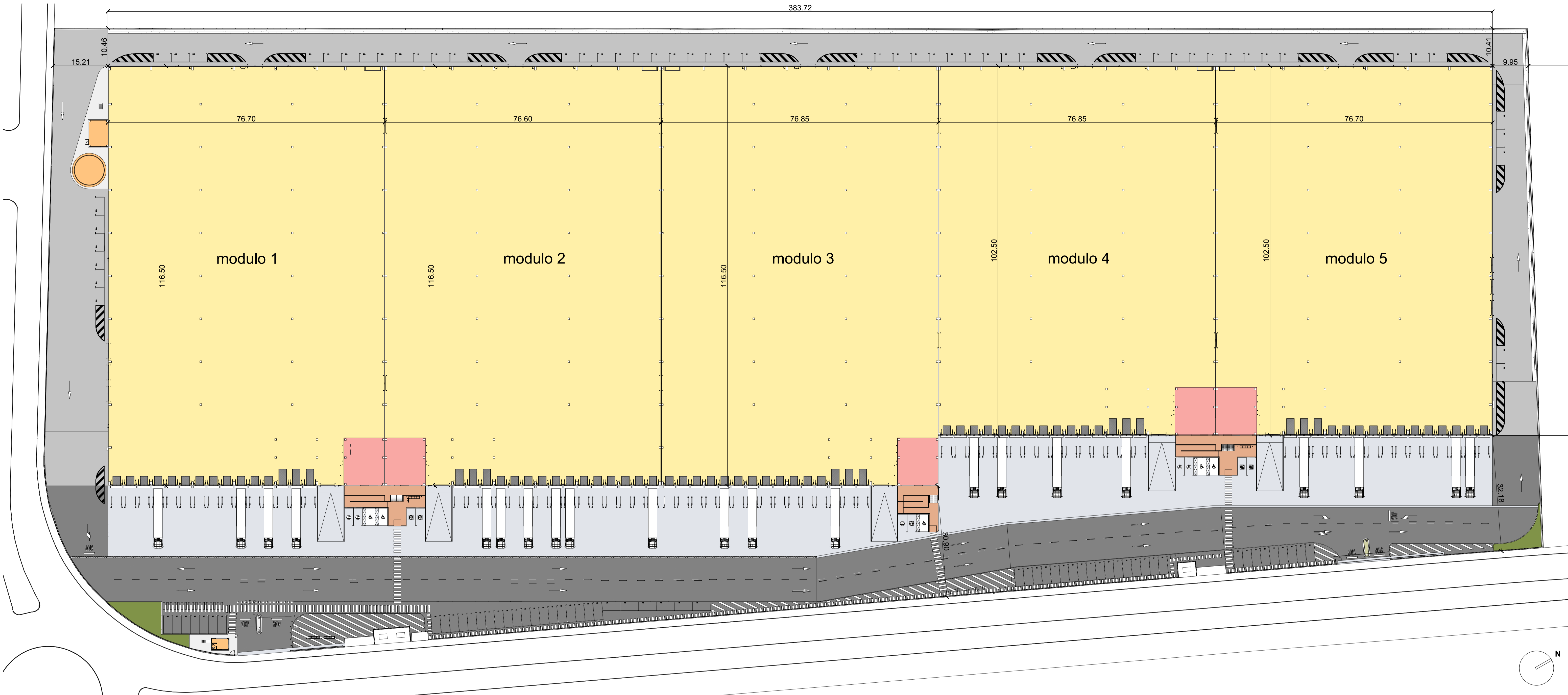
PLANTA GENERAL LAYOUT 1:500
